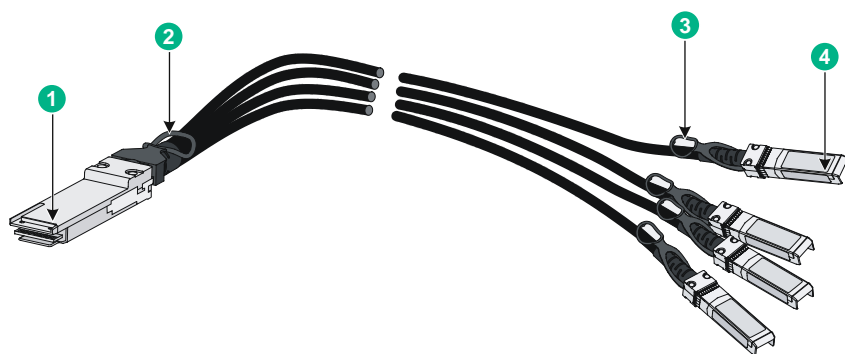
图4-6 100G QSFP28 to 4x25G SFP28 线缆
