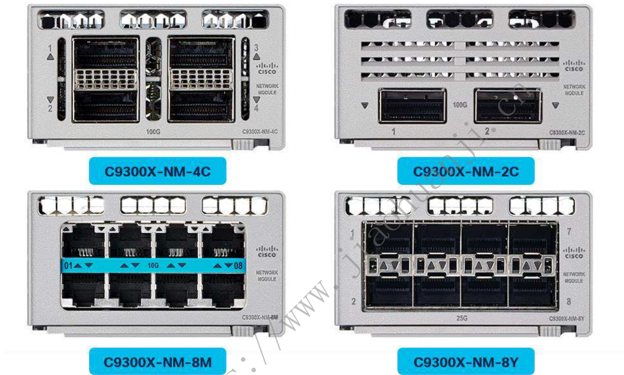
Figure 2. Cisco Catalyst 9300X Network Modules
