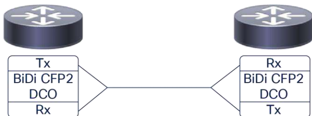
Figure 1. Single-fiber bidirectional communication with BiDi CFP2 DCO
